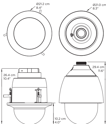
Flush mount
